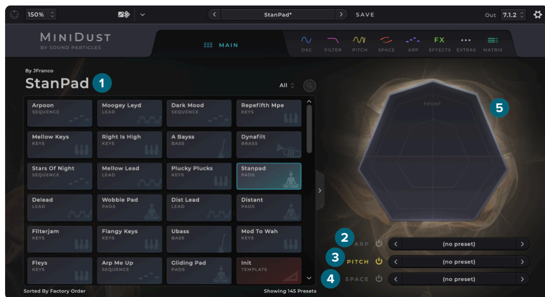
Main Page
