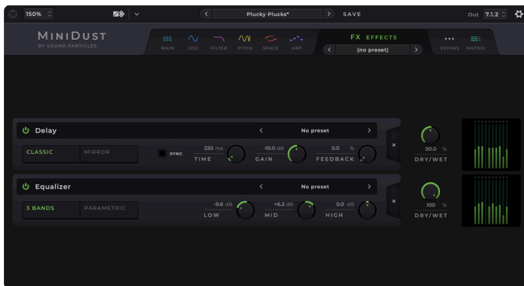
Effects Page
