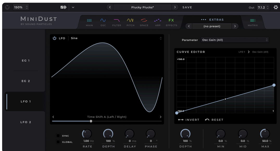
Extras Page
