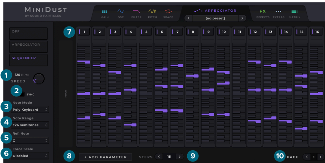
Sequencer
