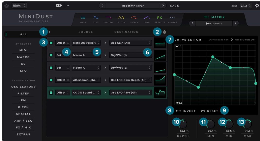
Matrix Page
