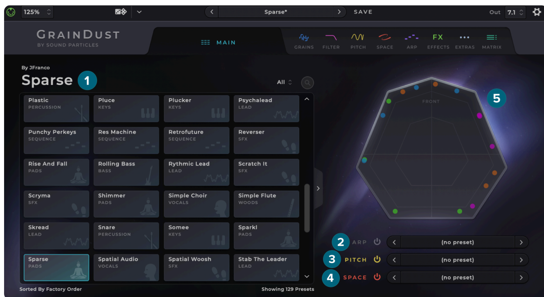
Main Page
