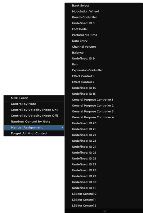
Control options
